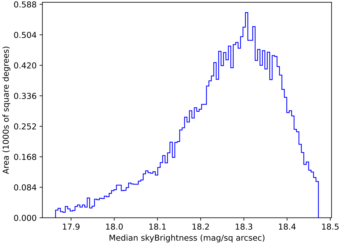
too_elab_r8_d3_gz_v3.4_10yrs Yr 1 y band: Median skyBrightness
