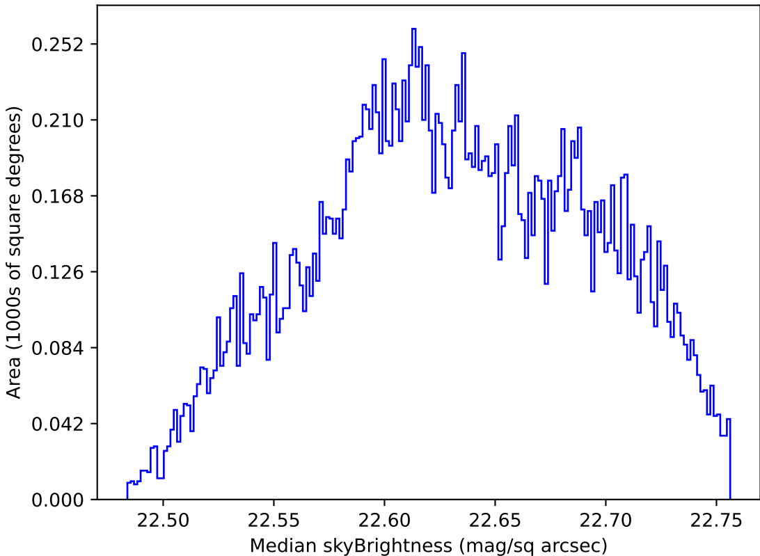
too_elab_r8_d3_gz_v3.4_10yrs Yr 1 u band: Median skyBrightness
