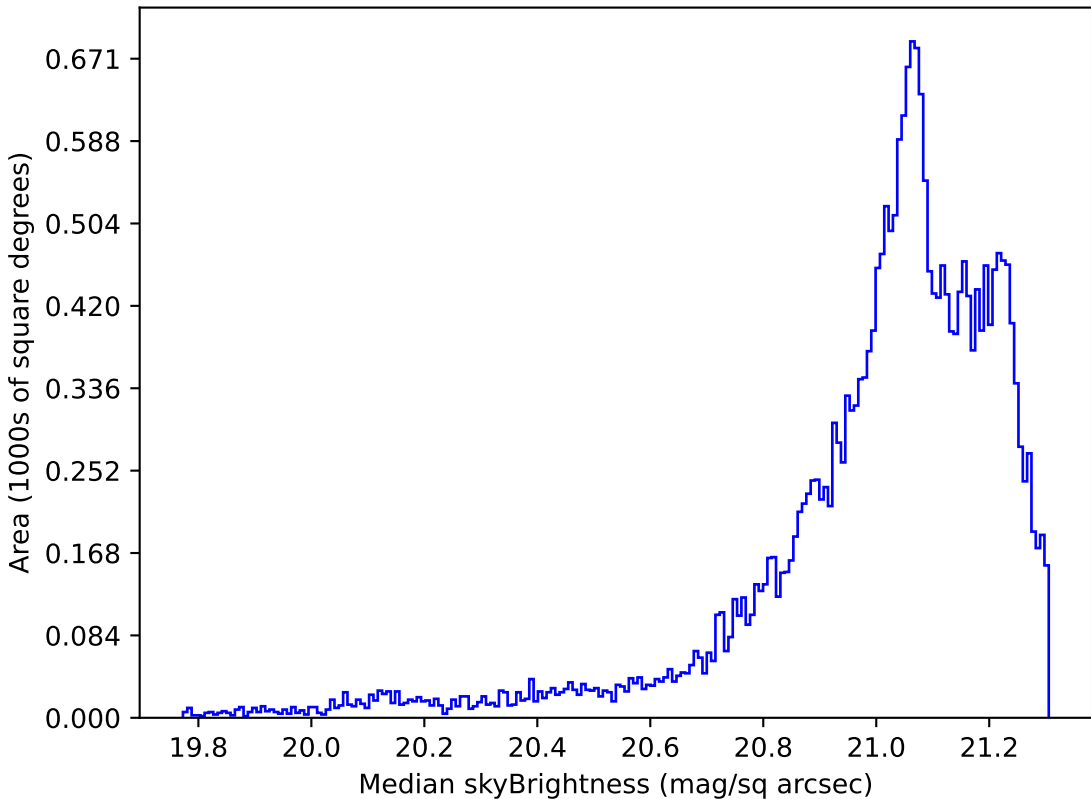
too_elab_r8_d3_gz_v3.4_10yrs Yr 1 r band: Median skyBrightness
