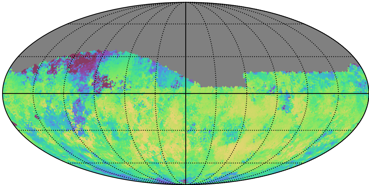
too_elab_r8_d3_gz_v3.4_10yrs Yr 1 i band: Median skyBrightness
