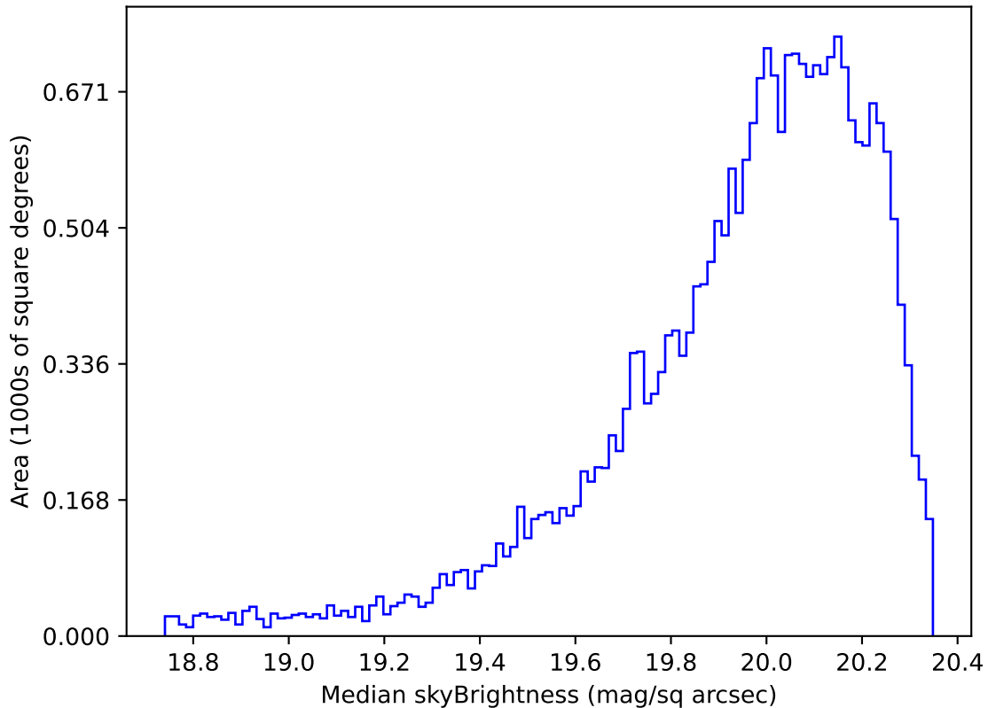
too_elab_r8_d3_gz_v3.4_10yrs Yr 1 i band: Median skyBrightness
