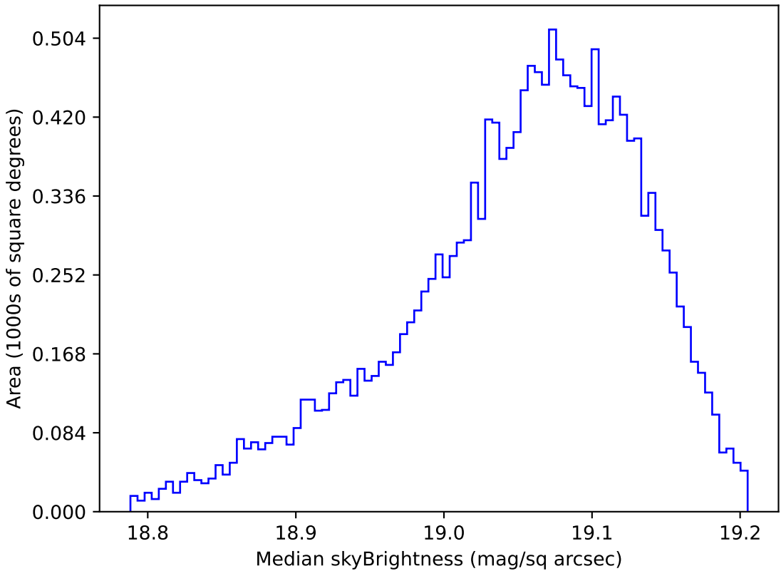
too_elab_r8_d3_gz_v3.4_10yrs WFD z band: Median skyBrightness
