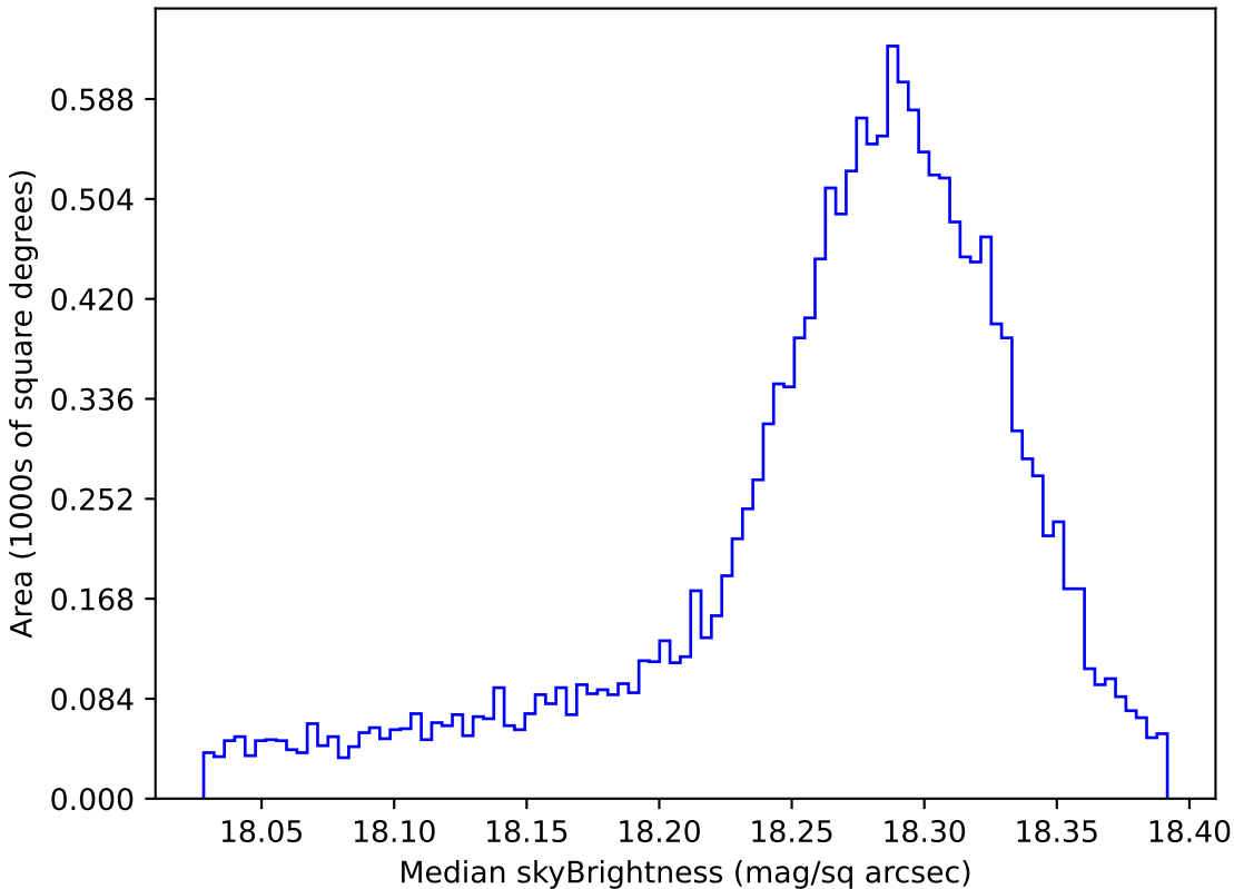
too_elab_r8_d3_gz_v3.4_10yrs WFD y band: Median skyBrightness
