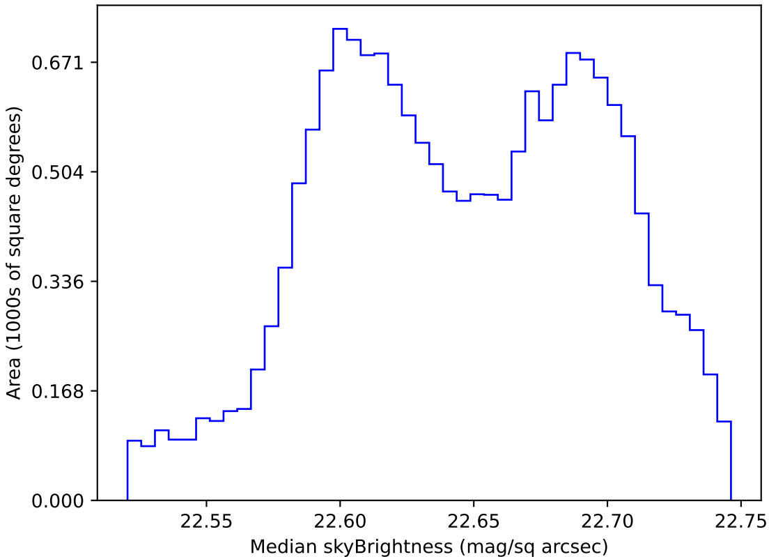
too_elab_r8_d3_gz_v3.4_10yrs WFD u band: Median skyBrightness
