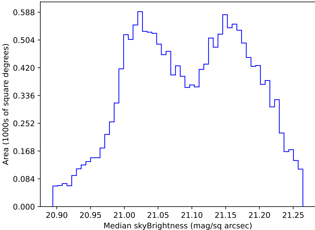
too_elab_r8_d3_gz_v3.4_10yrs WFD r band: Median skyBrightness
