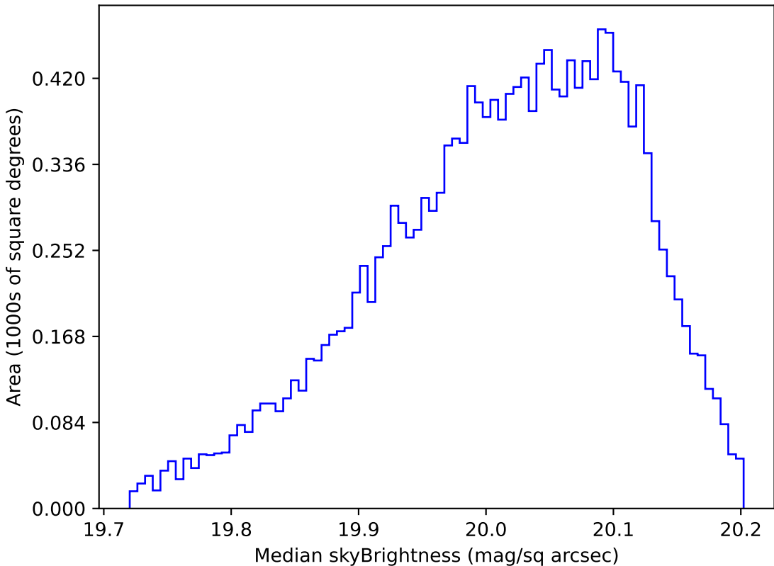
too_elab_r8_d3_gz_v3.4_10yrs WFD i band: Median skyBrightness
