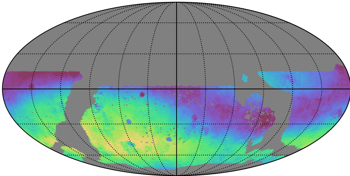
too_elab_r8_d3_gz_v3.4_10yrs WFD g band: Median skyBrightness
