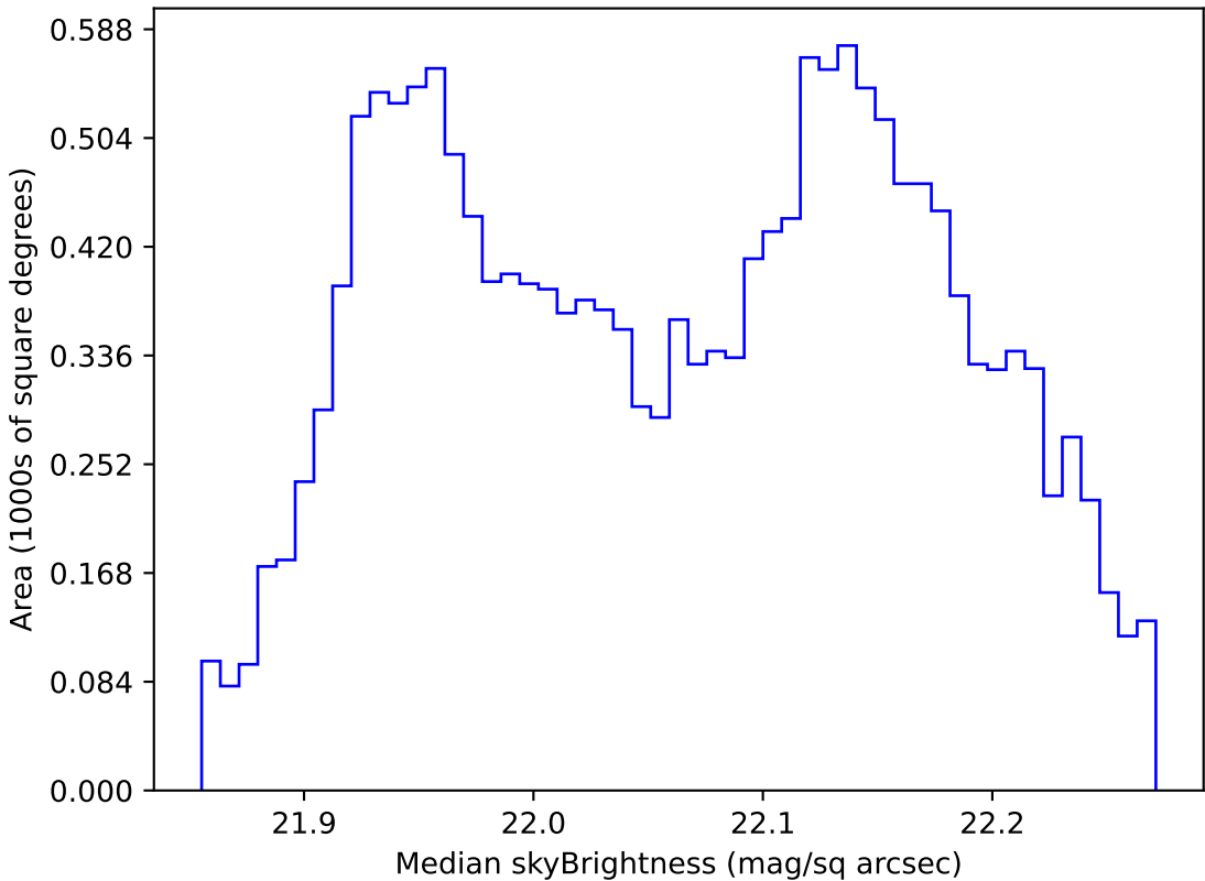
too_elab_r8_d3_gz_v3.4_10yrs WFD g band: Median skyBrightness
