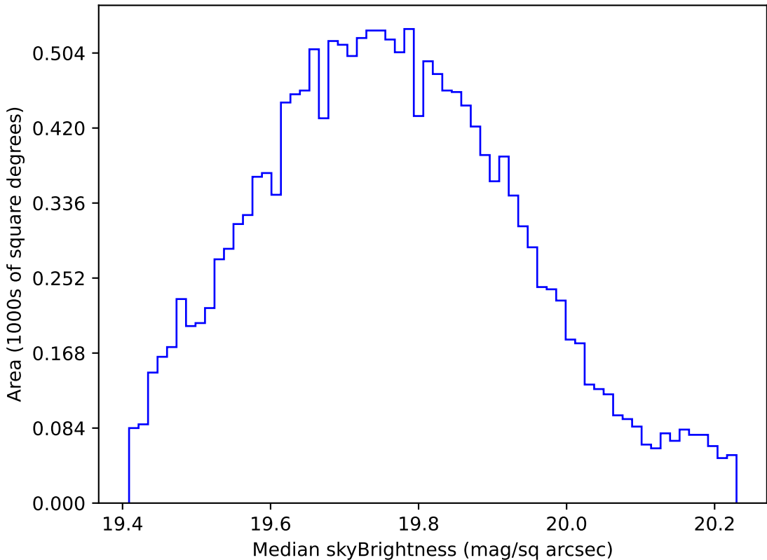
too_elab_r8_d3_gz_v3.4_10yrs WFD all bands: Median skyBrightness
