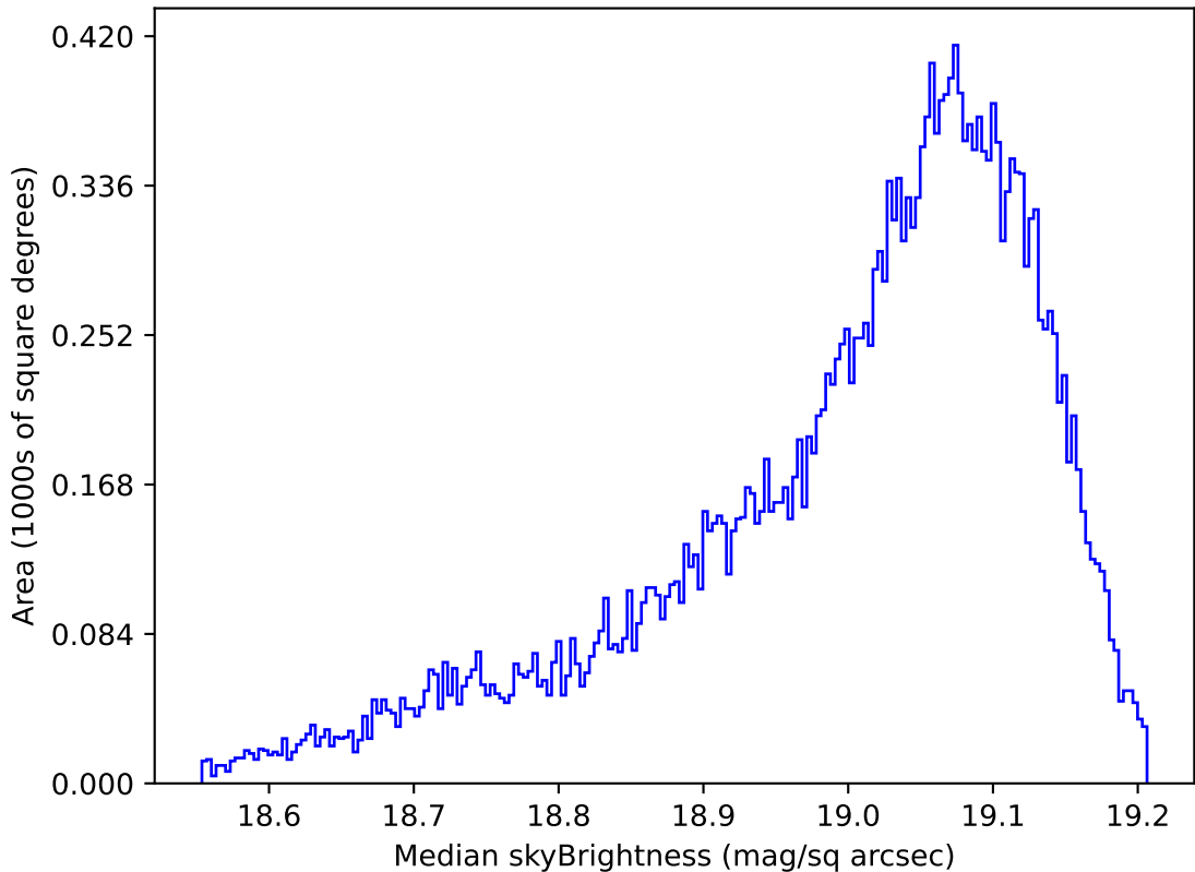
too_elab_r8_d3_gz_v3.4_10yrs All sky z band: Median skyBrightness
