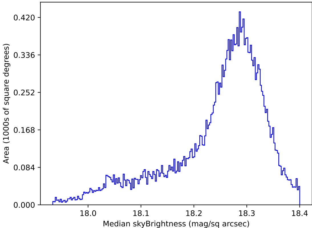
too_elab_r8_d3_gz_v3.4_10yrs All sky y band: Median skyBrightness
