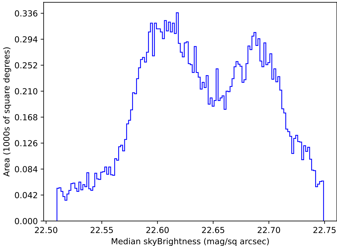
too_elab_r8_d3_gz_v3.4_10yrs All sky u band: Median skyBrightness
