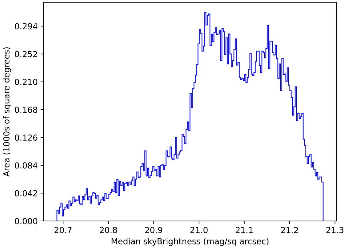
too_elab_r8_d3_gz_v3.4_10yrs All sky r band: Median skyBrightness
