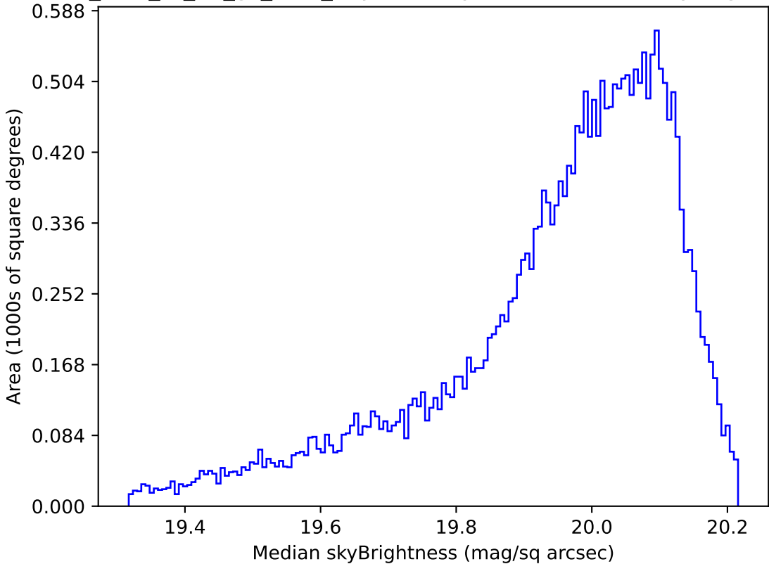
too_elab_r8_d3_gz_v3.4_10yrs All sky i band: Median skyBrightness
