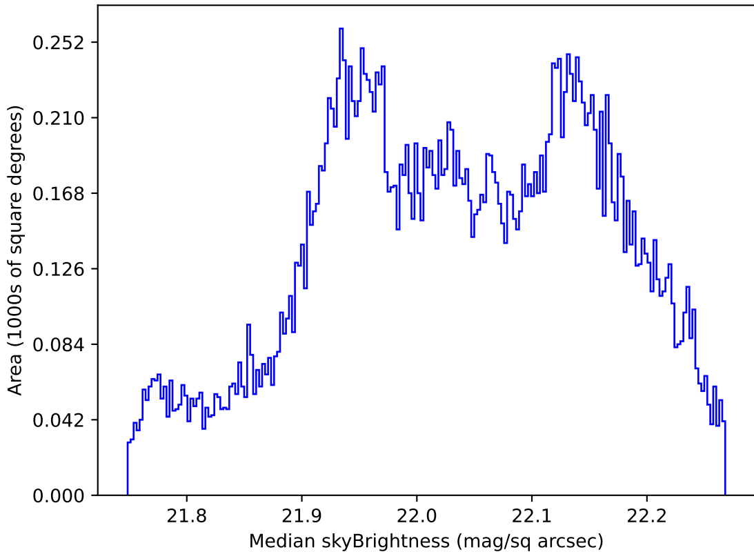
too_elab_r8_d3_gz_v3.4_10yrs All sky g band: Median skyBrightness
