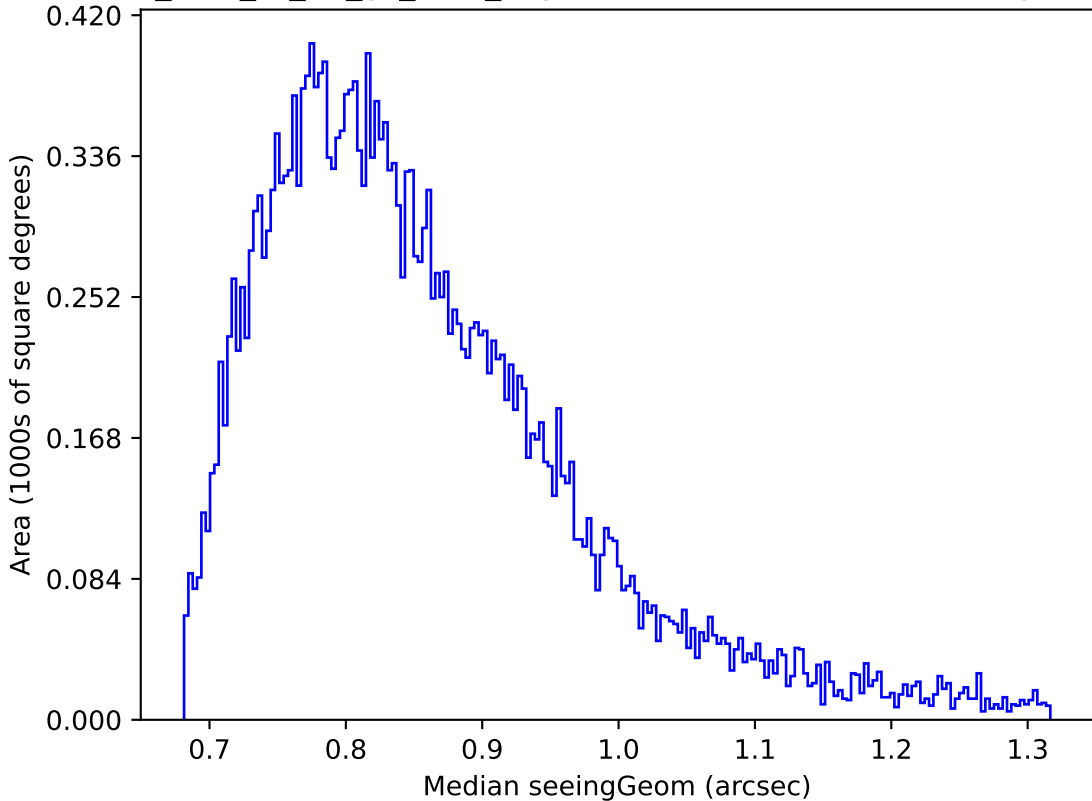
too_elab_r8_d3_gz_v3.4_10yrs Yr 1 z band: Median seeingGeom
