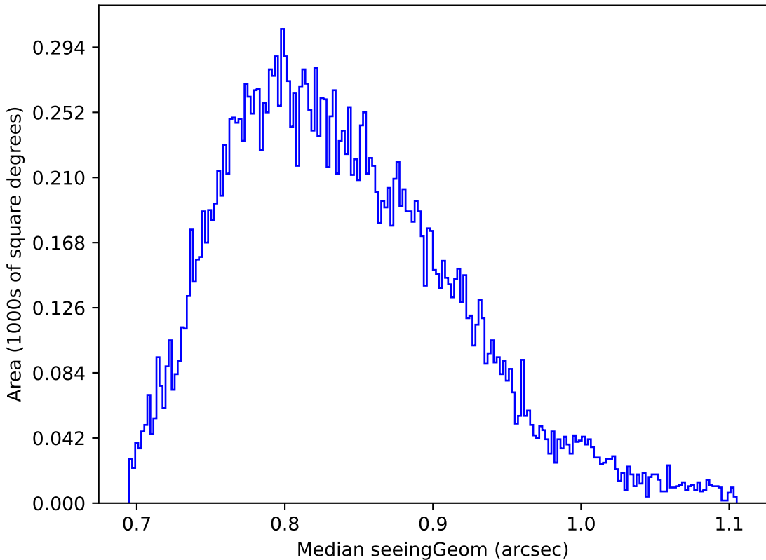
too_elab_r8_d3_gz_v3.4_10yrs Yr 1 y band: Median seeingGeom
