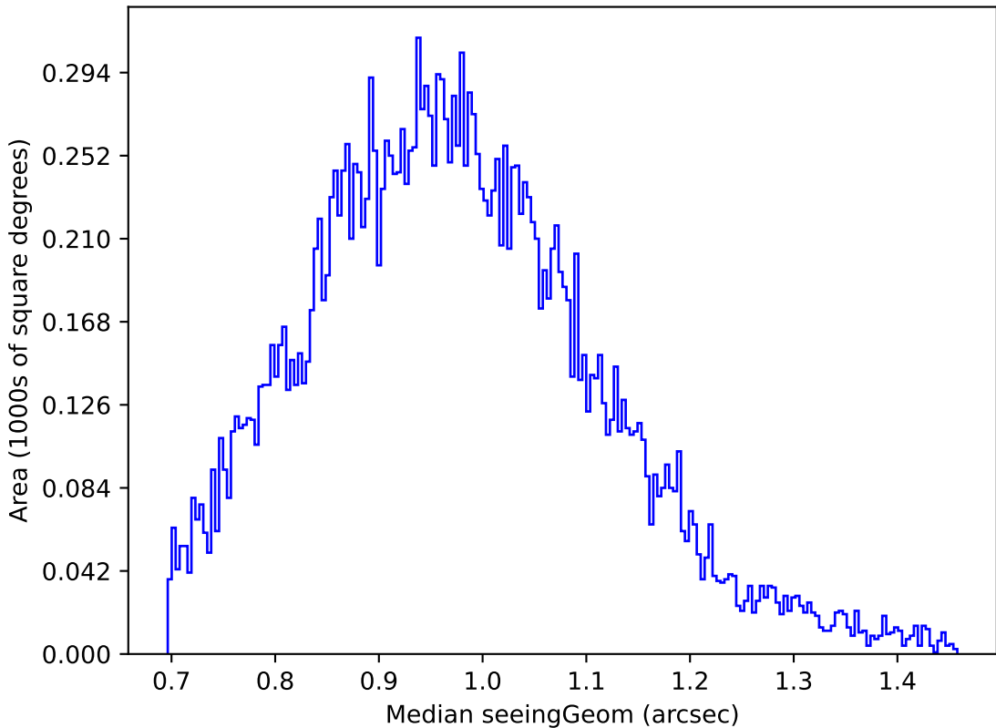
too_elab_r8_d3_gz_v3.4_10yrs Yr 1 u band: Median seeingGeom
