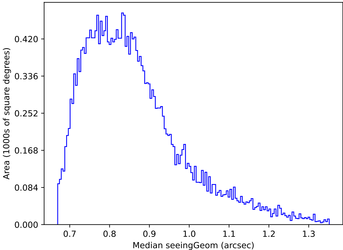
too_elab_r8_d3_gz_v3.4_10yrs Yr 1 r band: Median seeingGeom
