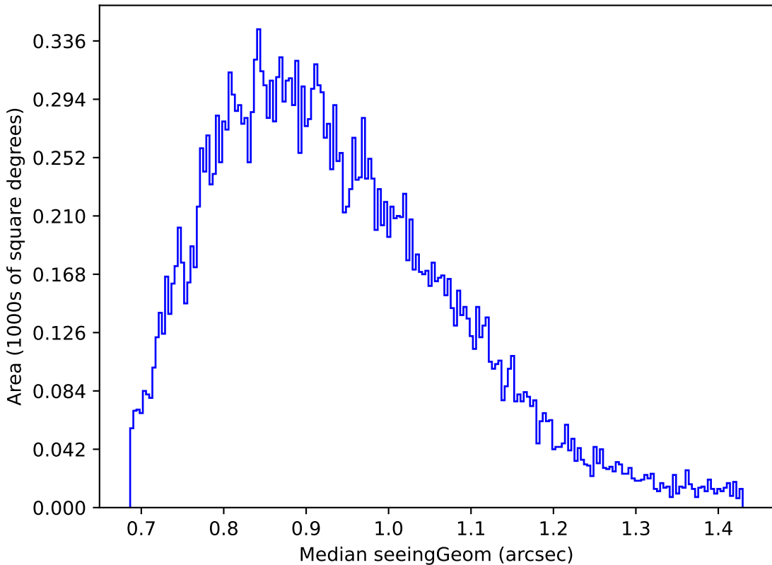
too_elab_r8_d3_gz_v3.4_10yrs Yr 1 g band: Median seeingGeom
