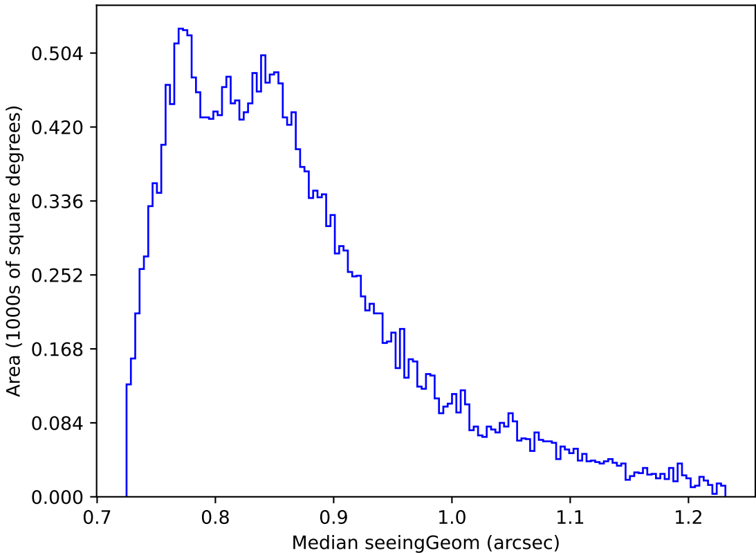
too_elab_r8_d3_gz_v3.4_10yrs Yr 1 all bands: Median seeingGeom
