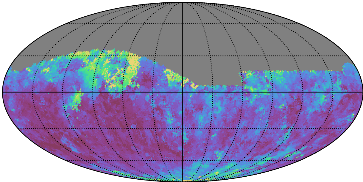
too_elab_r8_d3_gz_v3.4_10yrs Yr 1 z band: Median seeingEff
