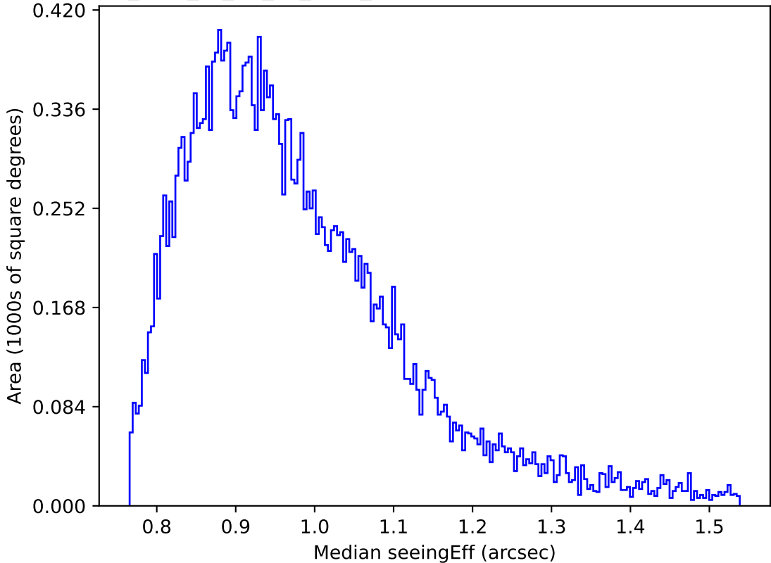
too_elab_r8_d3_gz_v3.4_10yrs Yr 1 z band: Median seeingEff
