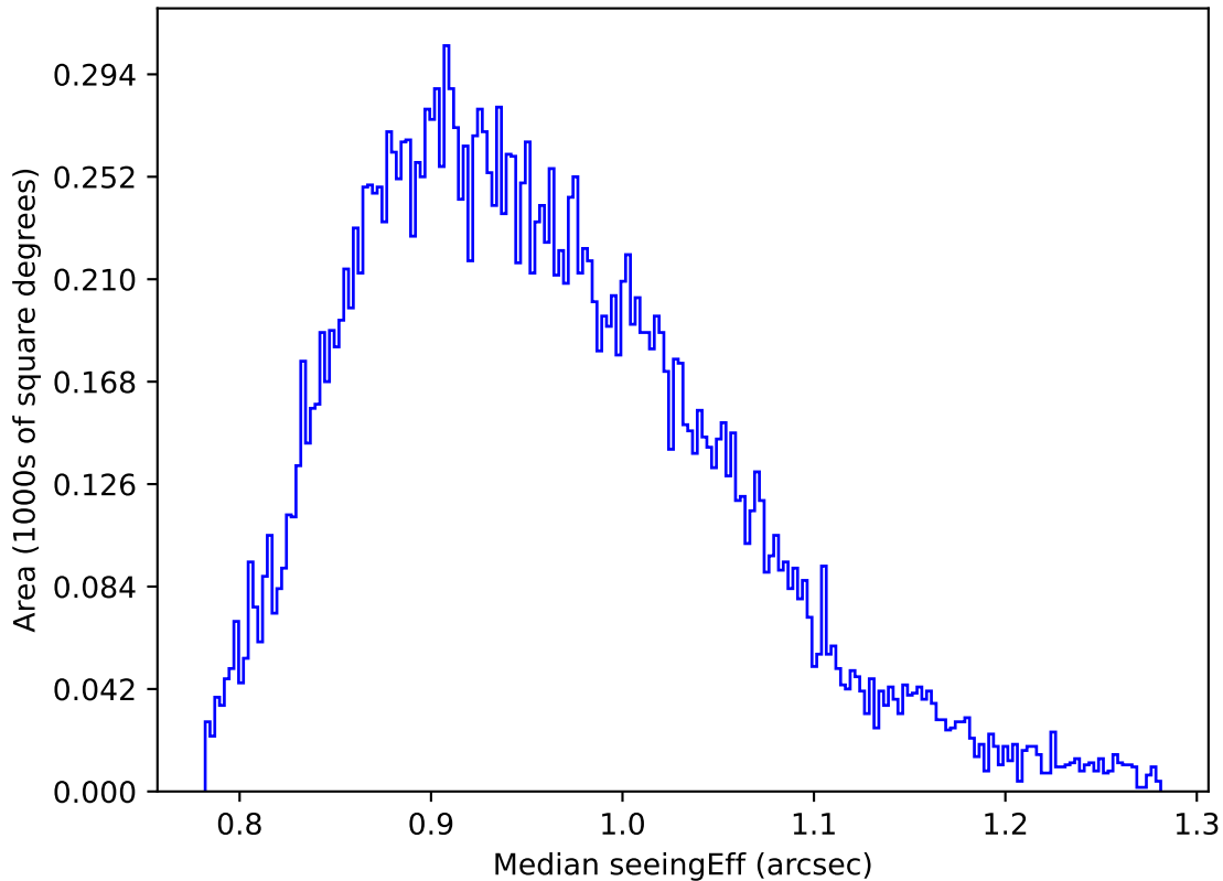
too_elab_r8_d3_gz_v3.4_10yrs Yr 1 y band: Median seeingEff
