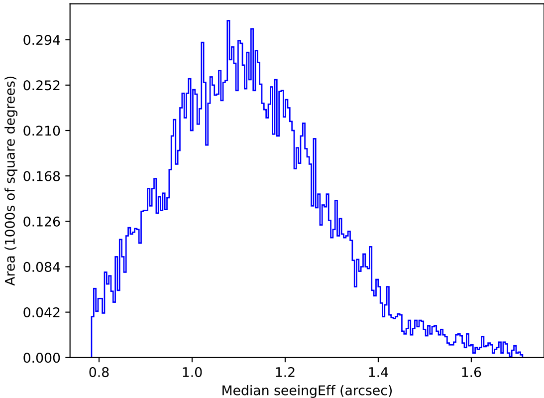
too_elab_r8_d3_gz_v3.4_10yrs Yr 1 u band: Median seeingEff
