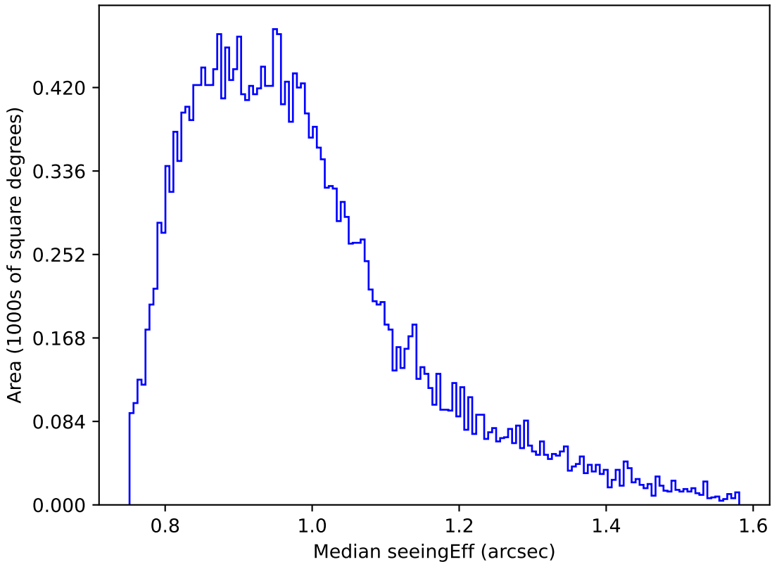
too_elab_r8_d3_gz_v3.4_10yrs Yr 1 r band: Median seeingEff
