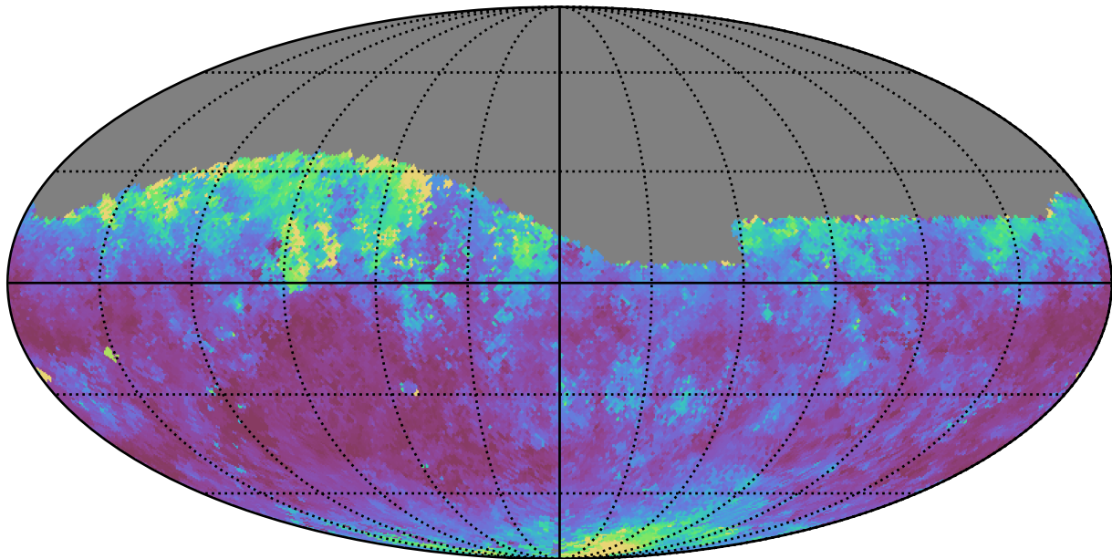
too_elab_r8_d3_gz_v3.4_10yrs Yr 1 i band: Median seeingEff
