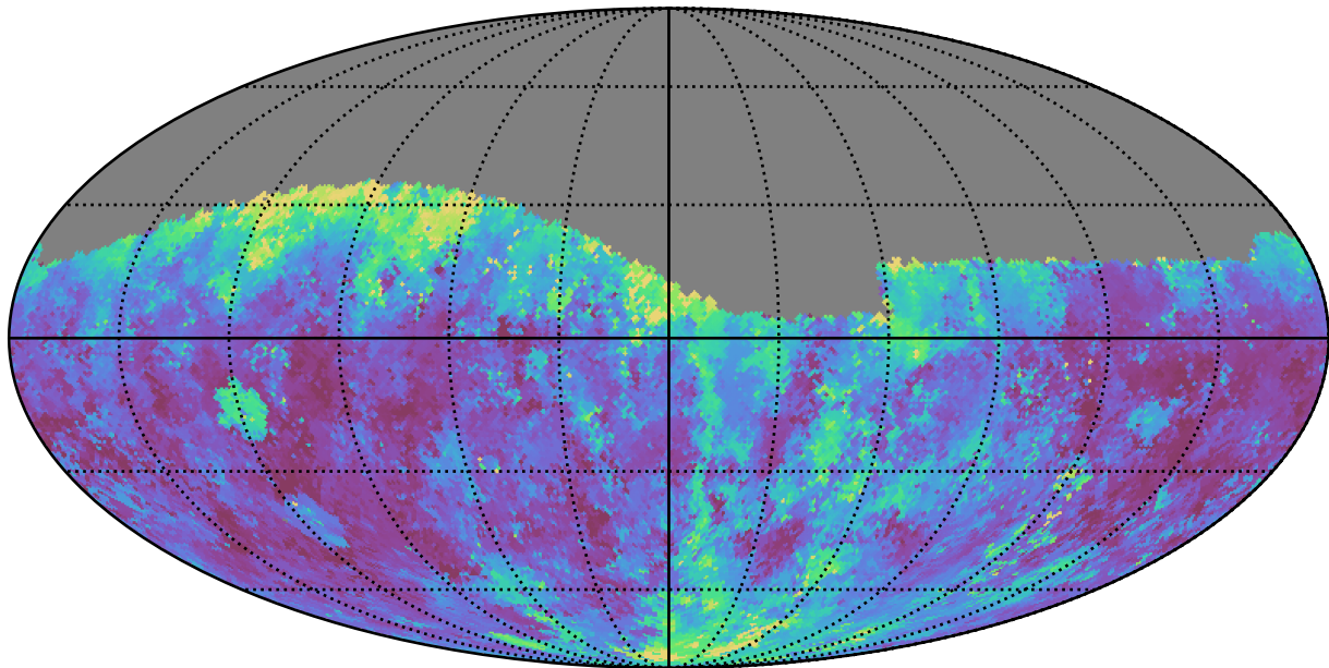
too_elab_r8_d3_gz_v3.4_10yrs Yr 1 g band: Median seeingEff
