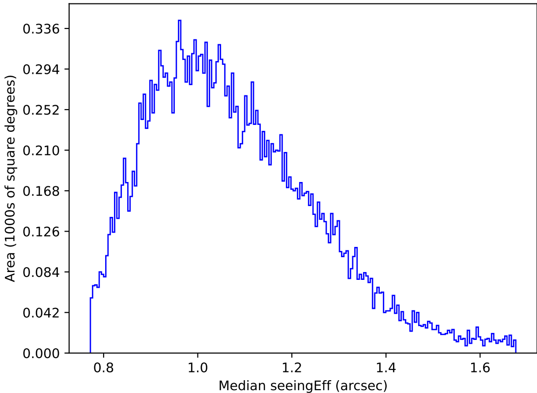
too_elab_r8_d3_gz_v3.4_10yrs Yr 1 g band: Median seeingEff
