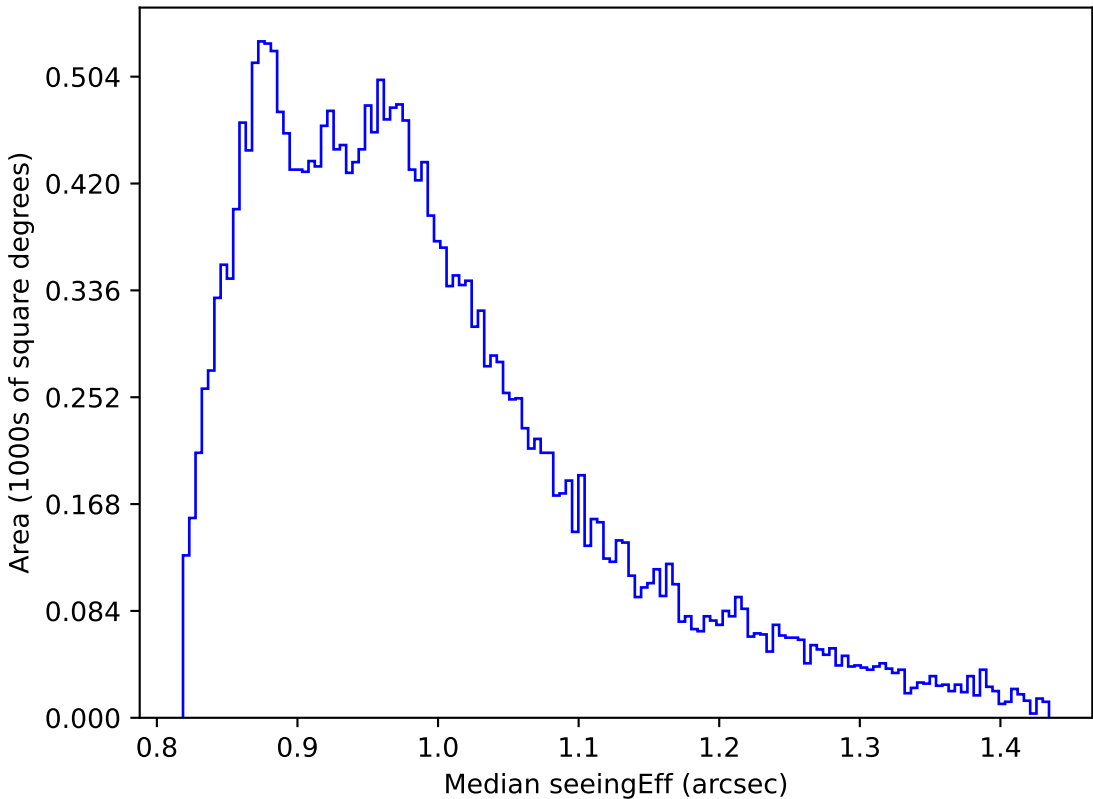
too_elab_r8_d3_gz_v3.4_10yrs Yr 1 all bands: Median seeingEff
