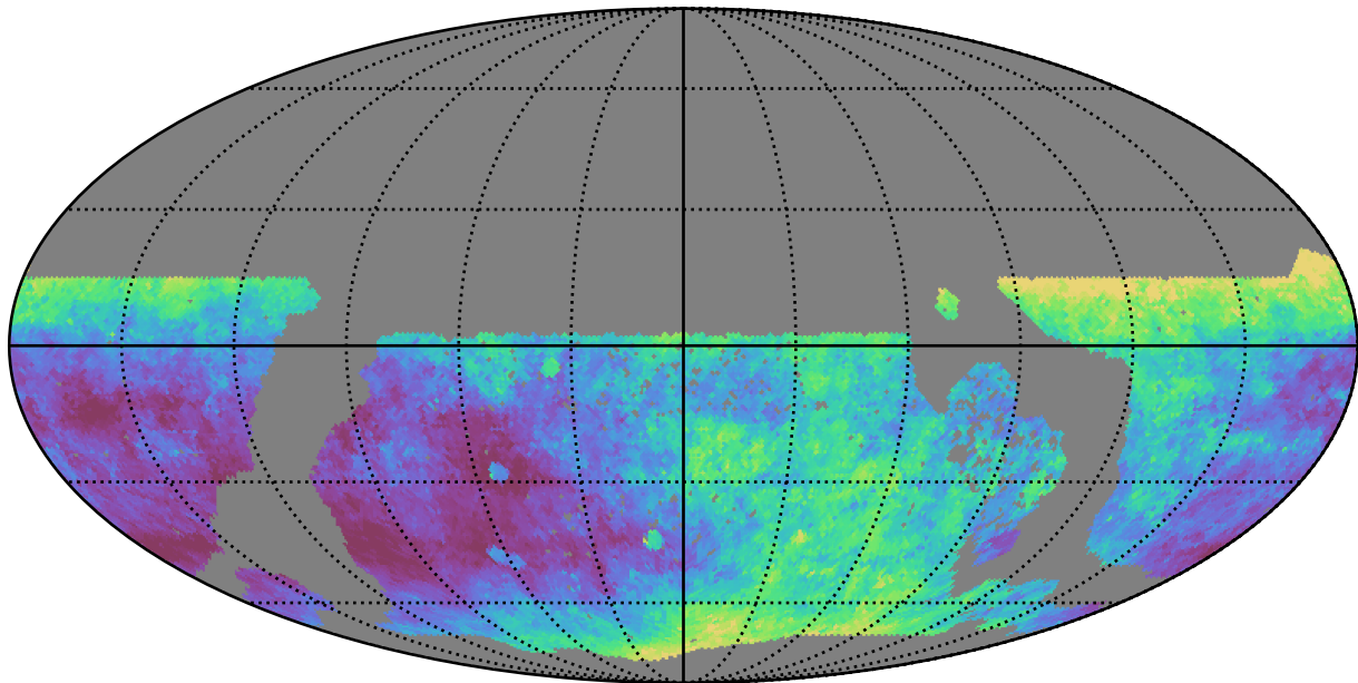
too_elab_r8_d3_gz_v3.4_10yrs WFD z band: Median seeingEff
