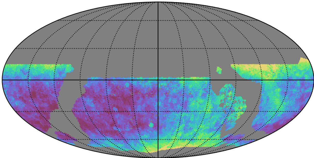
too_elab_r8_d3_gz_v3.4_10yrs WFD y band: Median seeingEff
