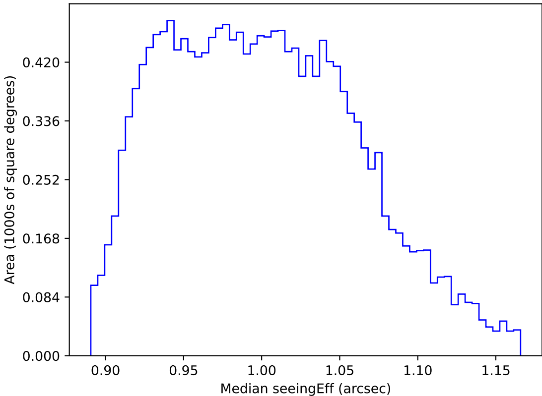
too_elab_r8_d3_gz_v3.4_10yrs WFD y band: Median seeingEff
