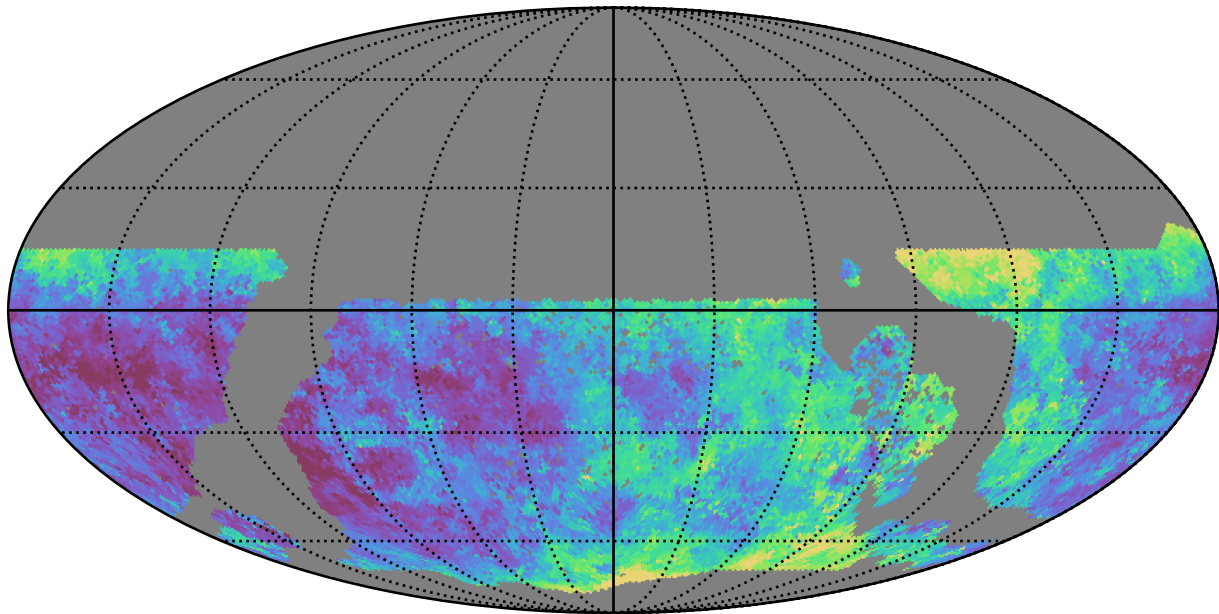
too_elab_r8_d3_gz_v3.4_10yrs WFD u band: Median seeingEff
