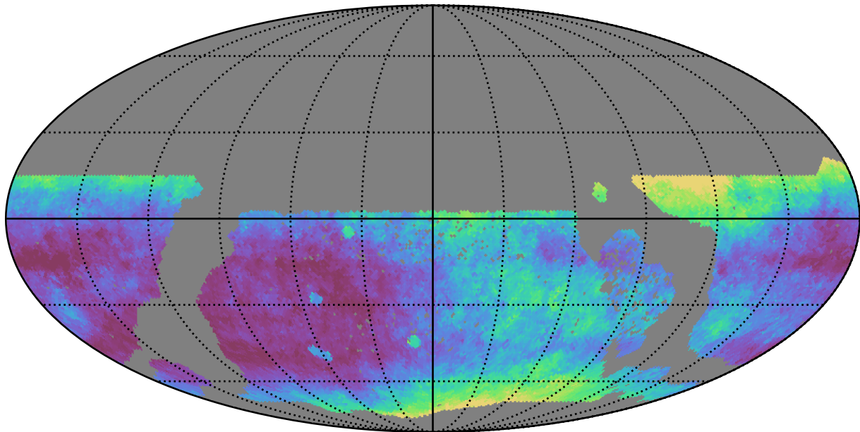
too_elab_r8_d3_gz_v3.4_10yrs WFD r band: Median seeingEff
