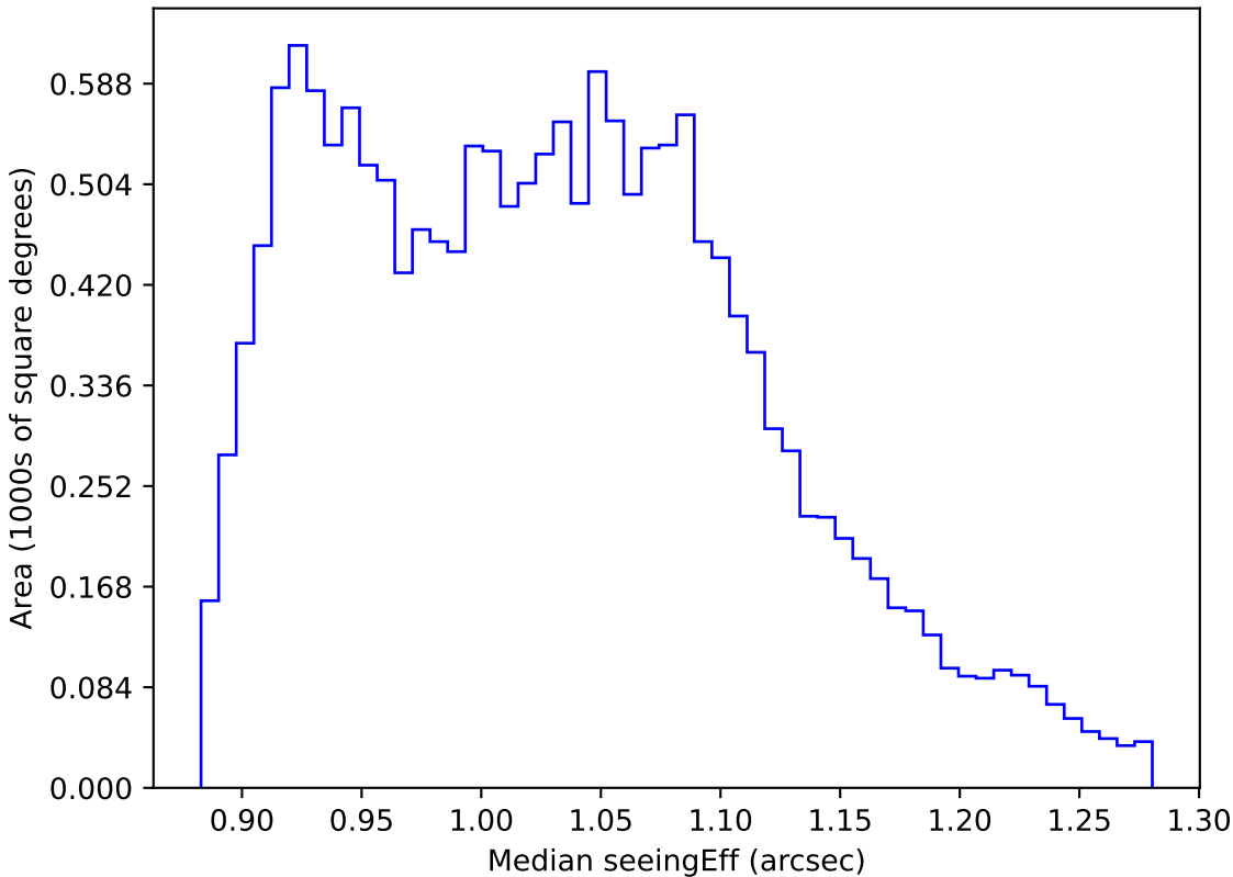
too_elab_r8_d3_gz_v3.4_10yrs WFD r band: Median seeingEff
