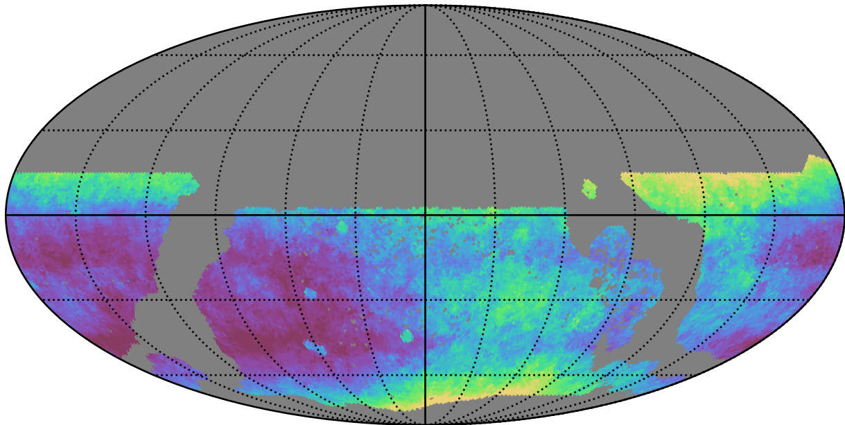
too_elab_r8_d3_gz_v3.4_10yrs WFD i band: Median seeingEff
