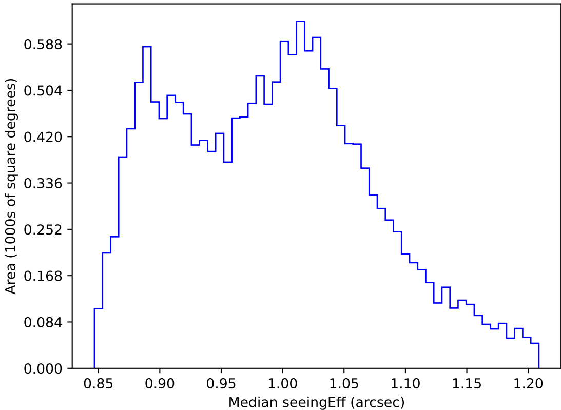
too_elab_r8_d3_gz_v3.4_10yrs WFD i band: Median seeingEff
