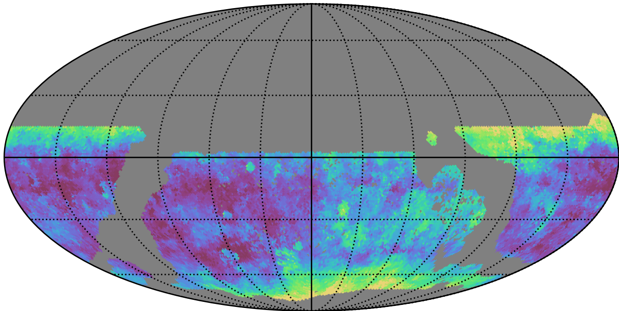
too_elab_r8_d3_gz_v3.4_10yrs WFD g band: Median seeingEff
