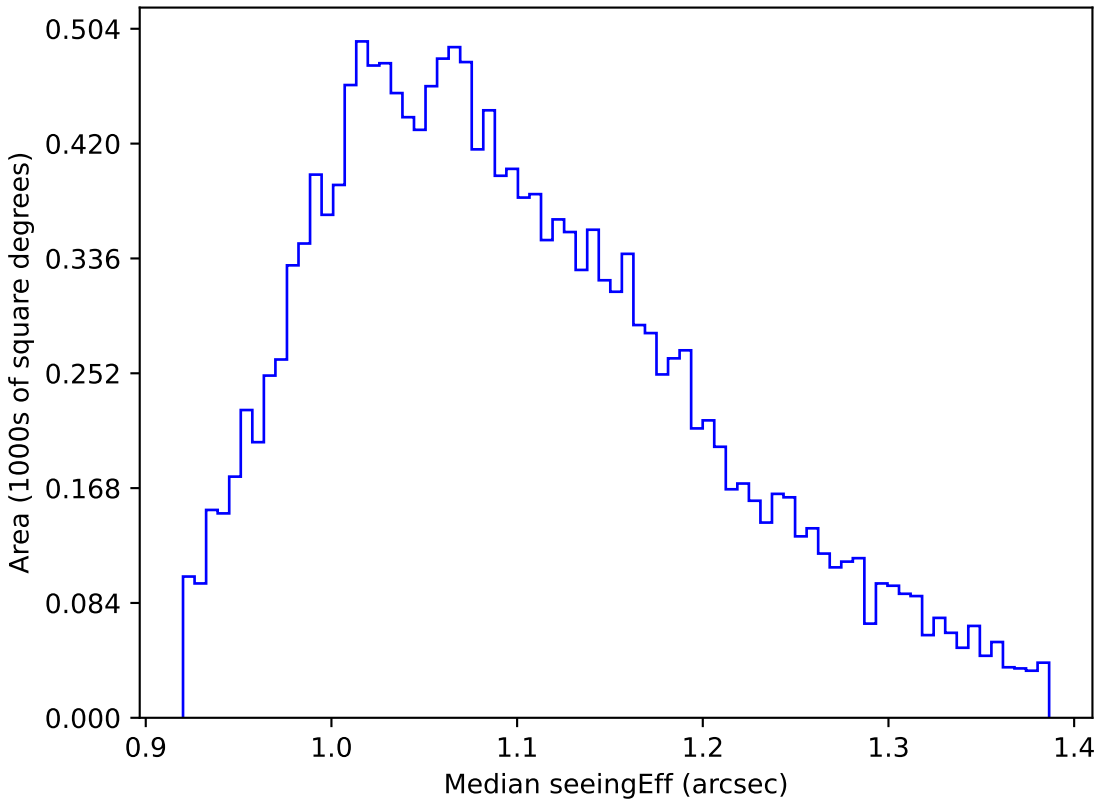
too_elab_r8_d3_gz_v3.4_10yrs WFD g band: Median seeingEff
