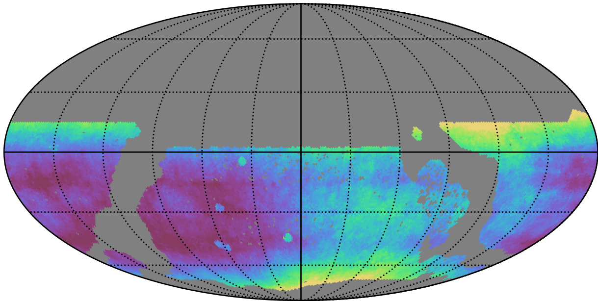
too_elab_r8_d3_gz_v3.4_10yrs WFD all bands: Median seeingEff
