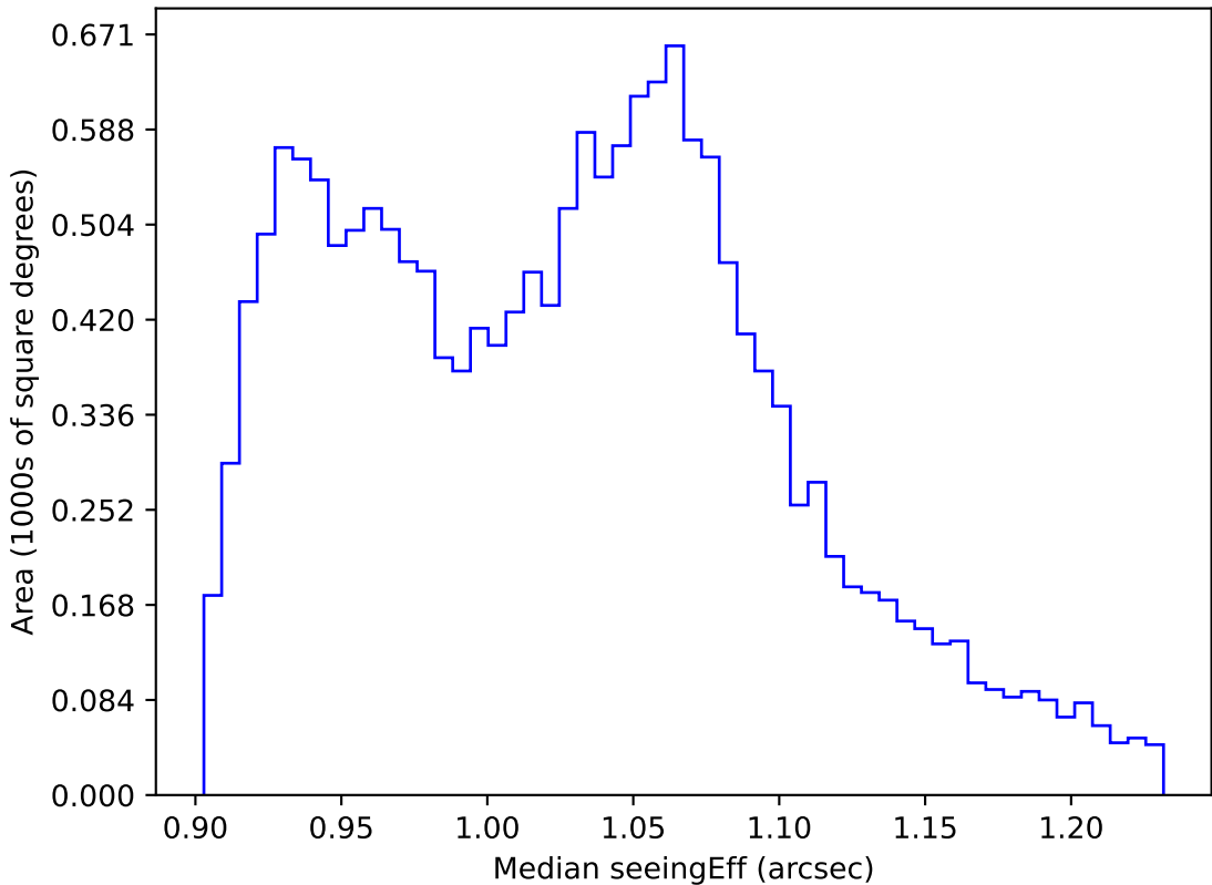
too_elab_r8_d3_gz_v3.4_10yrs WFD all bands: Median seeingEff
