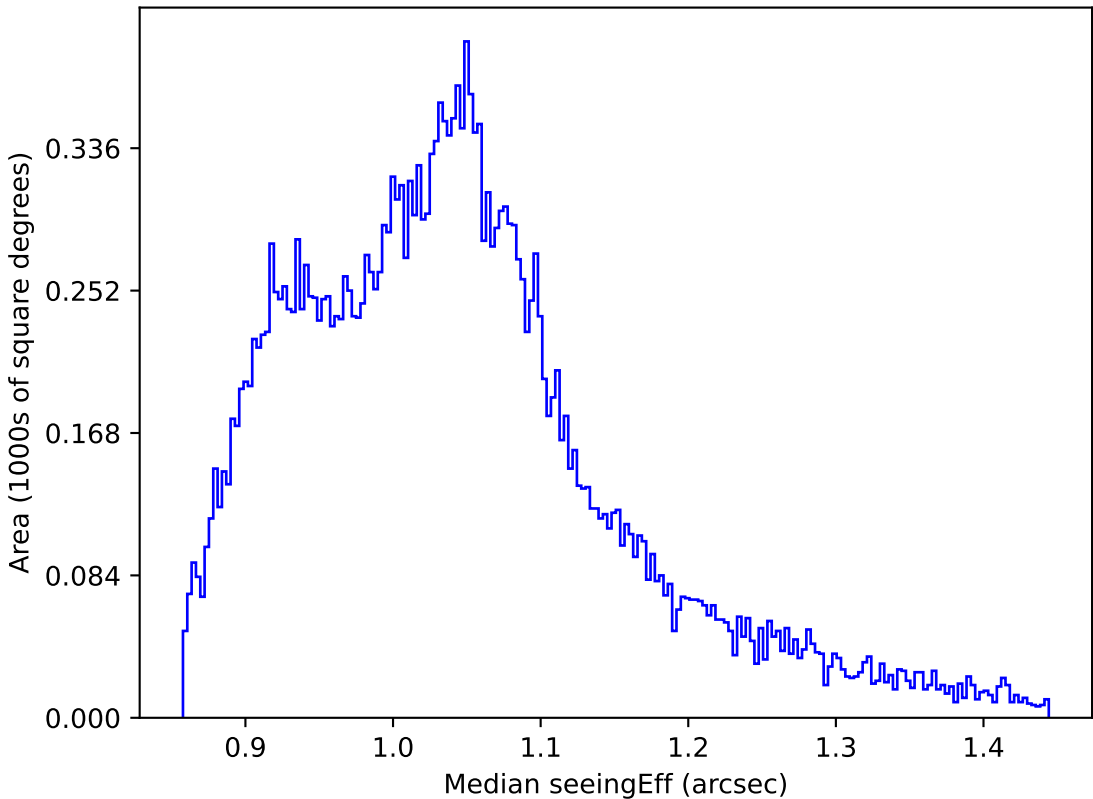
too_elab_r8_d3_gz_v3.4_10yrs All sky z band: Median seeingEff
