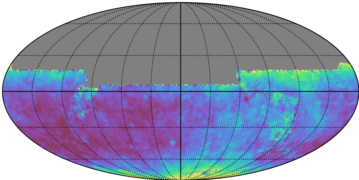
too_elab_r8_d3_gz_v3.4_10yrs All sky y band: Median seeingEff
