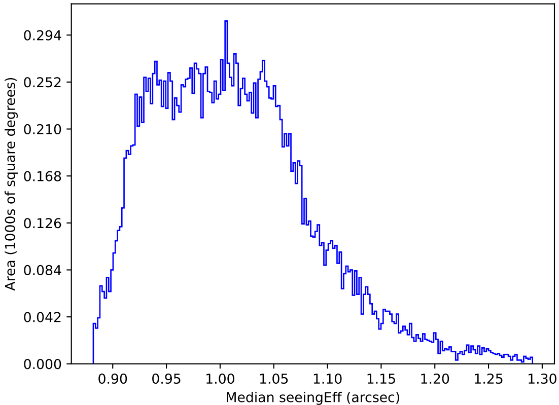
too_elab_r8_d3_gz_v3.4_10yrs All sky y band: Median seeingEff
