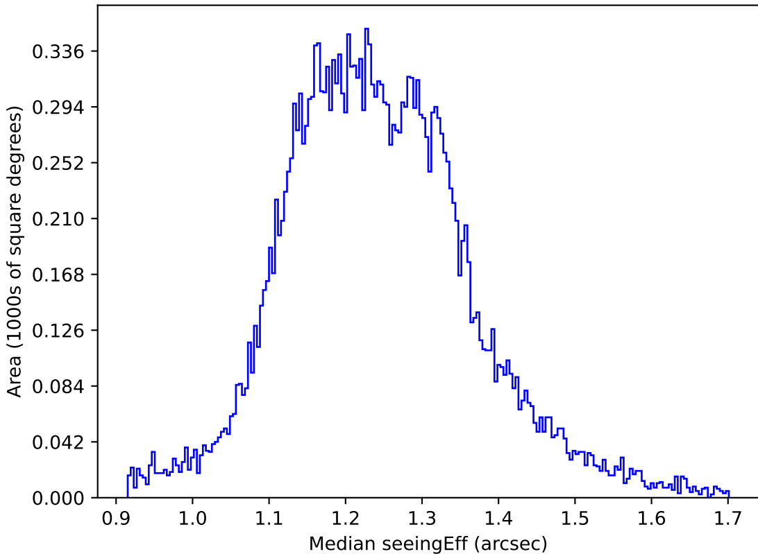
too_elab_r8_d3_gz_v3.4_10yrs All sky u band: Median seeingEff
